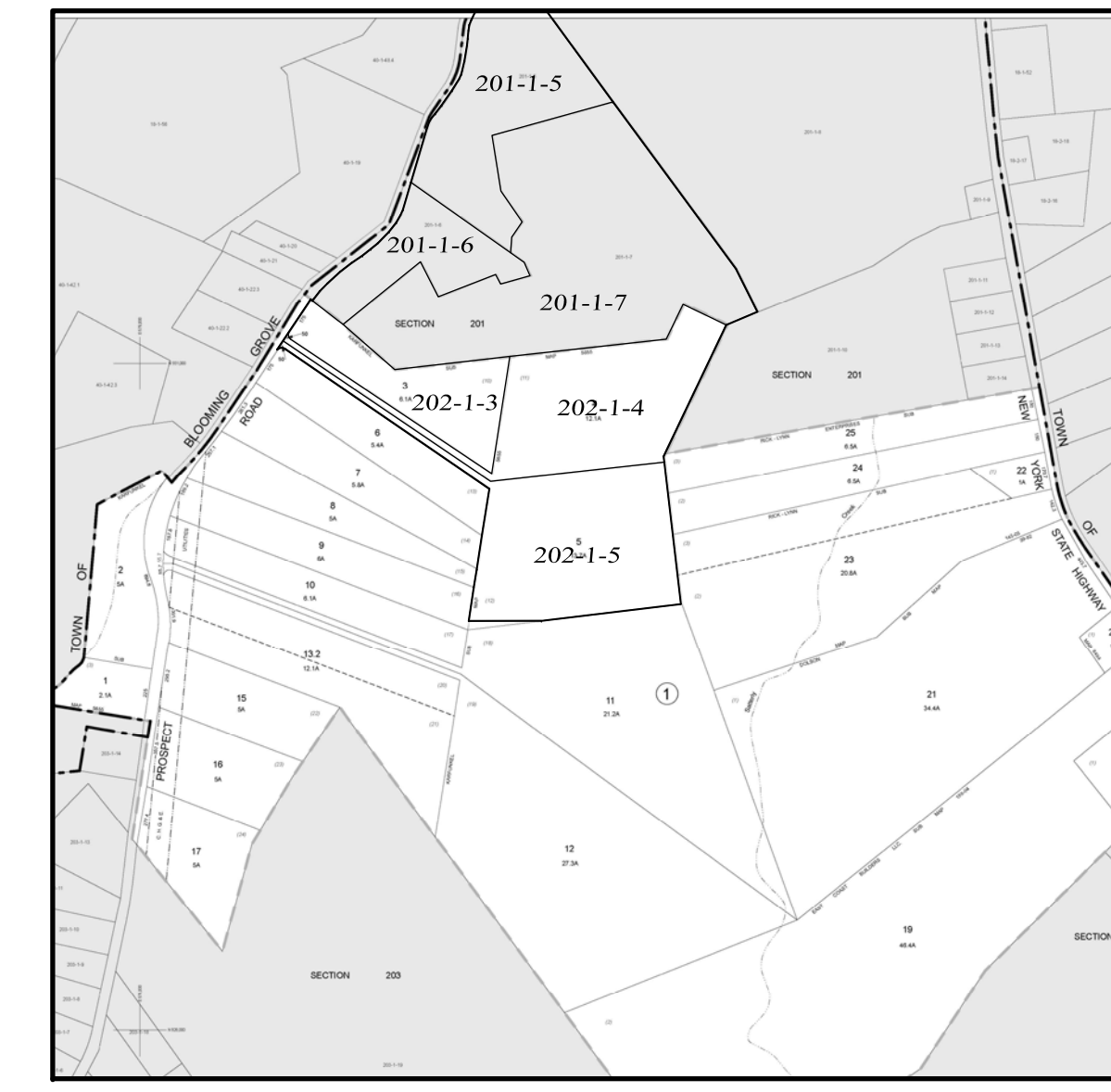
LOCATION MAP SCALE: 1" = 800'
