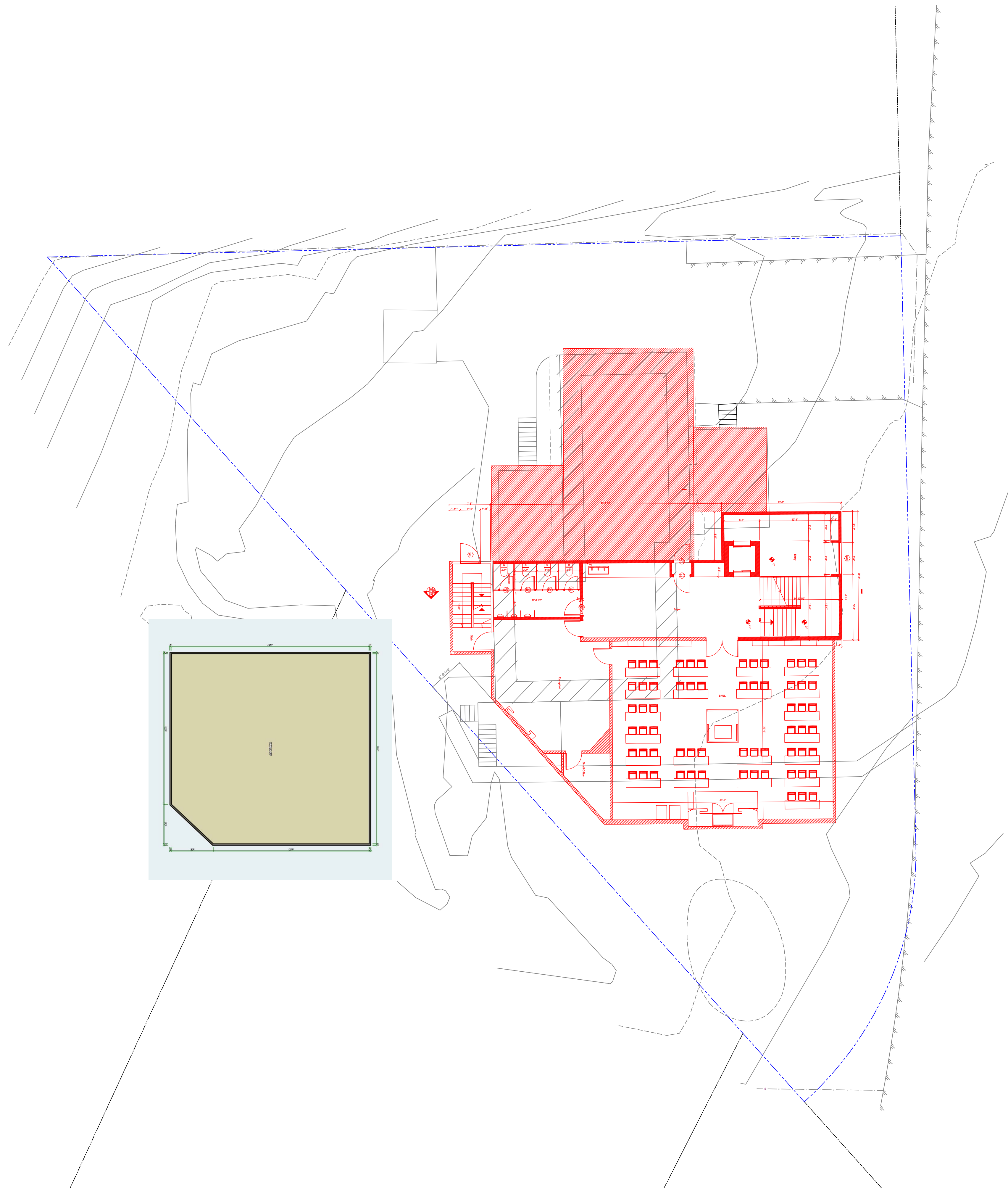
1 PLAN VIEW - SITE PLAN 3/32" - 1' - 0"
